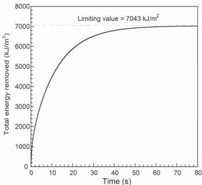
Figure 3-20 Energy removed from the glass vs. time.
