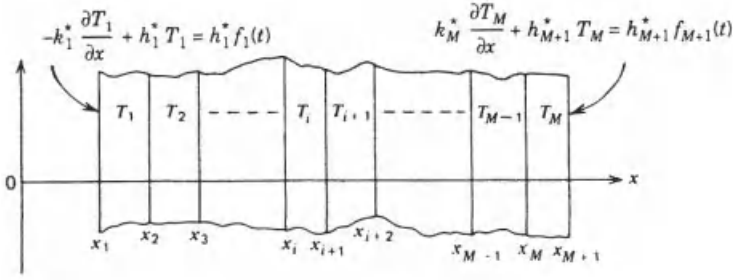
Figure 10-1 M -layer composite region.
