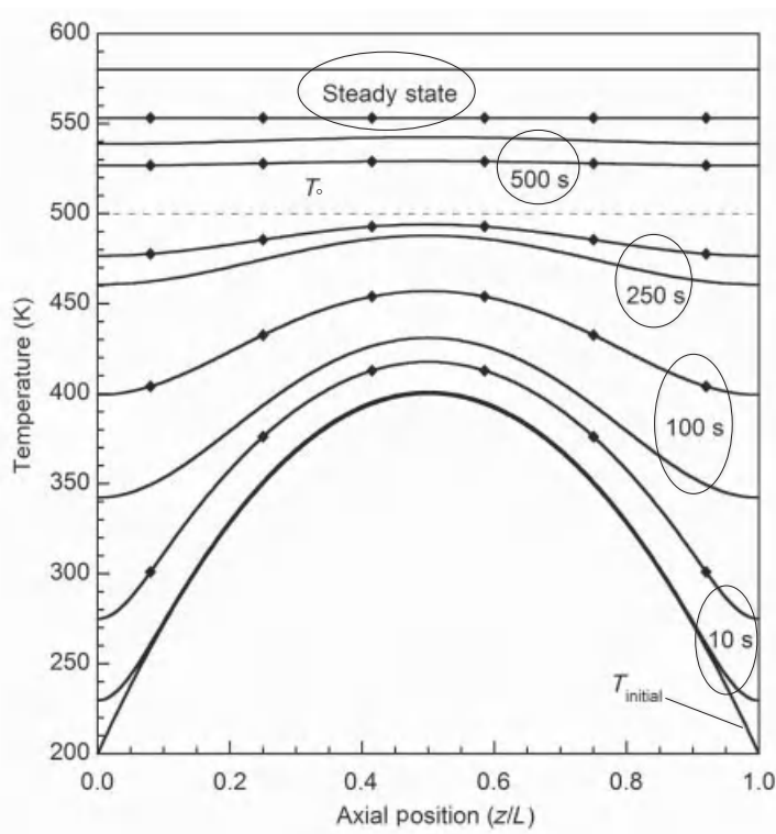
Figure 4-7 Axial temperature profiles for various times, including the initial and steady-state profiles. The dashed line at 500 K represents the convective fluid temperature. For each time, two profiles are presented that correspond to the centerline ( r=0 ) and the outer surface ( r=b ), with the latter marked by the diamonds.
