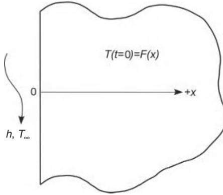
Figure 6-1 One-dimensional heat conduction in a semi-infinite medium.
