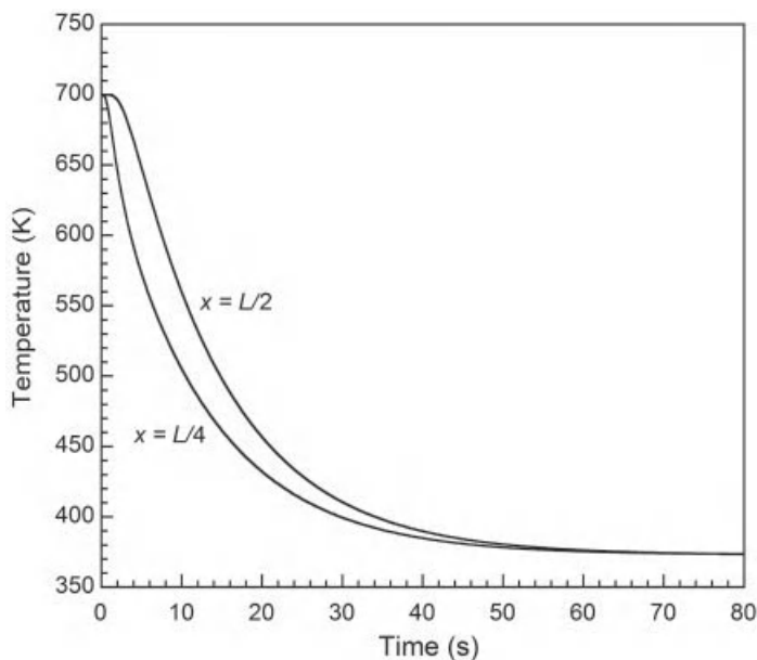
Figure 3-17 Temperature profile as function of time.
