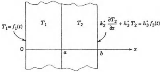
Figure 10-2 Two-layer slab with perfect thermal contact at the interface.
