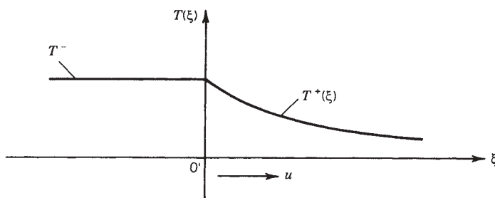
Figure 11-4 Quasi-stationary temperature distribution around a moving surface heat source.
