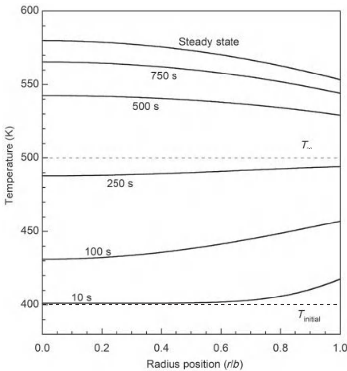
Figure 4-6 Radial temperature profiles at z = L/2 for various times, including the initial and steady-state profiles. The dashed line at 500 K represents the convective fluid temperature.
