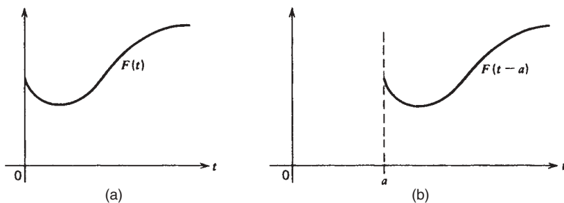
Figure 9-2 Translation of a function F(t) : (a) the function F(t) and (b) the translation of F(t) from t=0 to t=a .
