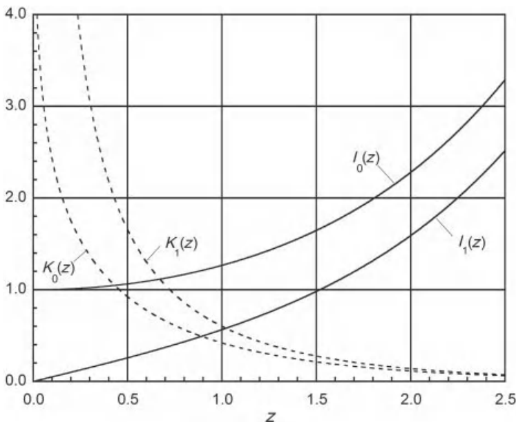
Figure 2-2 Modified Bessel functions of the first and second kind.
