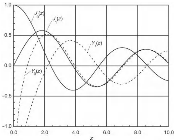
Figure 2-1 Bessel functions of the first and second kind.
