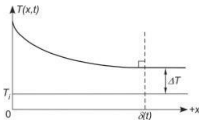
Figure 13-4 Thermal penetration distance in semi-infinite medium with internal energy generation.
