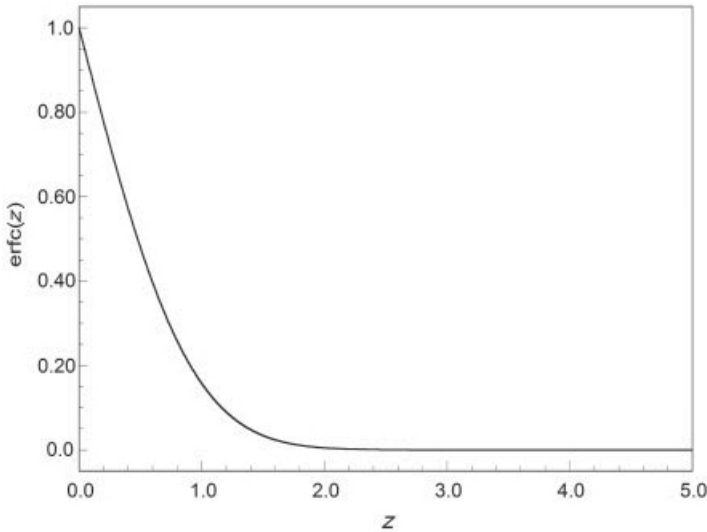
Figure 9-5 Behavior of the complementary error function.
