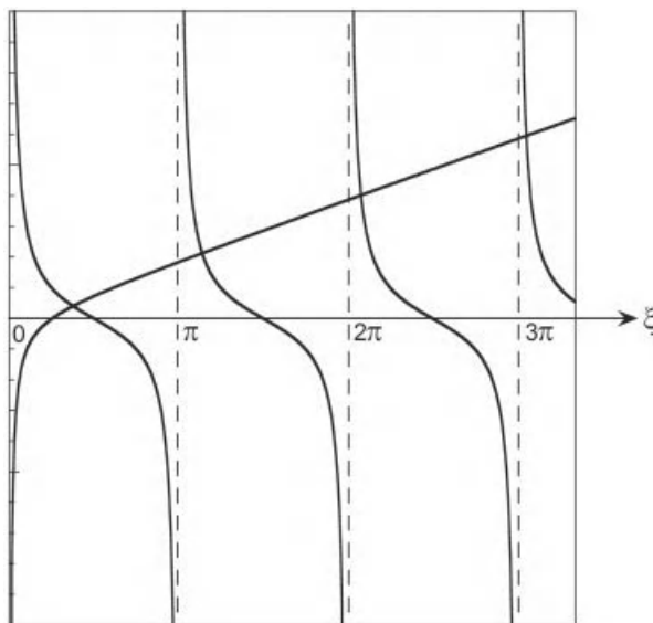
Figure 2-4 Graphical representation of the roots of equations (2-101).
