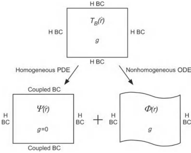
Figure 3-10 Superposition for nonhomogeneous pde.
