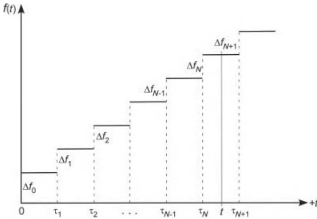
Figure 7-3 Stepwise varying boundary condition function f(t) .
