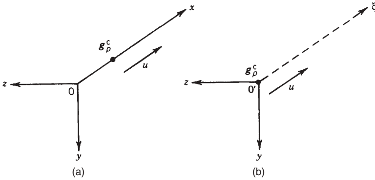
Figure 11-1 Moving point heat source: (a) fixed coordinates x, y, z and (b) moving coordinates \xi, y, z .
