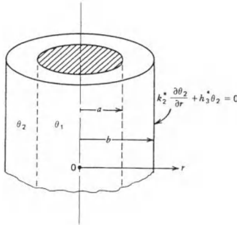
Figure 10-4 Two-layer cylinder with perfect thermal contact at the interface.
