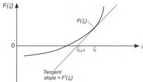
Figure 2-6 Newton–Raphson method.
