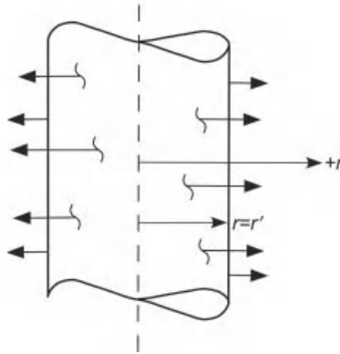
Figure 8-3 One-dimensional planar heat source in the cylindrical system.
