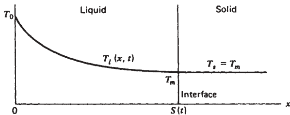
Figure 12-4 Melting in a half-space. Single-phase problem.
