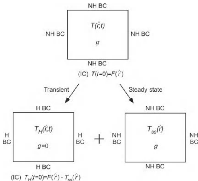
Figure 3-7 Superposition for general nonhomogeneous (NH) problem.
