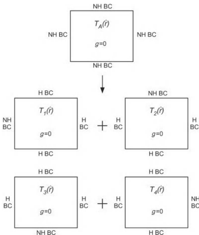
Figure 3-9 Superposition for nonhomogeneous BCs.
