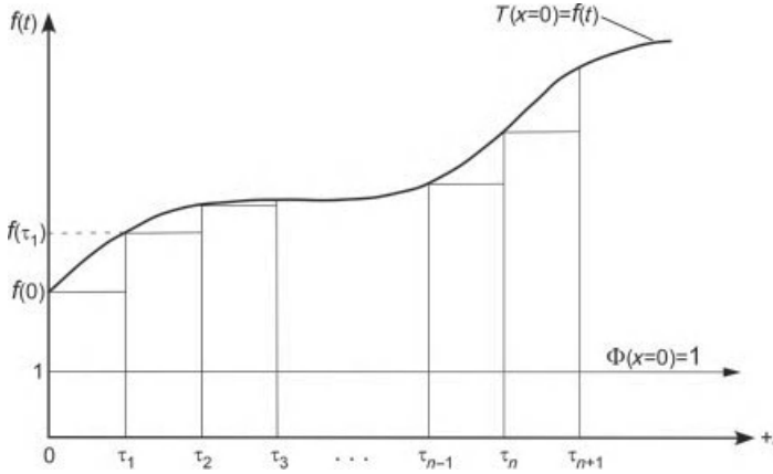
Figure 7-1 Time-dependent boundary condition at x = 0 .
