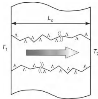
Figure 16-5 Diffusion of heat due to a temperature gradient.
