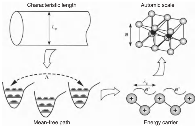
Figure 16-1 Length scales from the largest to smallest dimensions relevant to conduction heat transfer.
