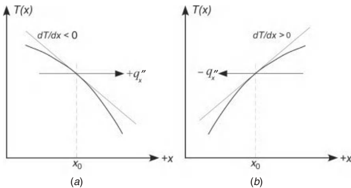
Figure 1-1 Fourier's law illustrated for a (a) positive heat flux and (b) a negative heat flux.
