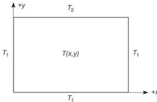
Figure 3-1 Heat conduction in a rectangular solid.
