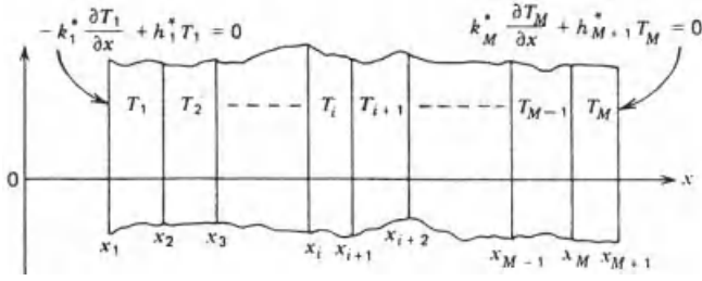
Figure 10-3 M -layer composite region.
