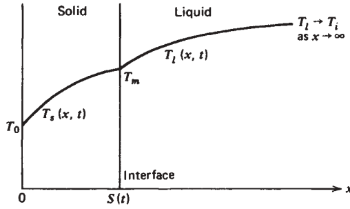
Figure 12-5 Solidification in a half-space. Two-phase problem.
