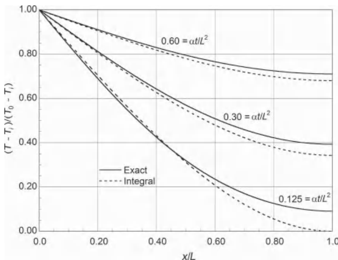
Figure 13-5 Comparison of exact and approximate temperature profiles for a slab of thickness L .
