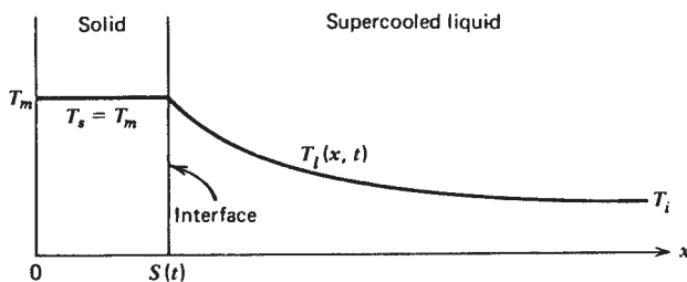
Figure 12-3 Solidification of supercooled liquid in a half-space.
