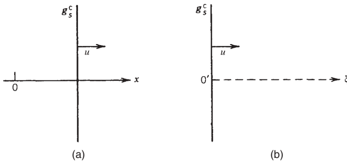
Figure 11-3 Moving plane surface heat source: (a) fixed coordinate x and (b) moving coordinate \xi .
