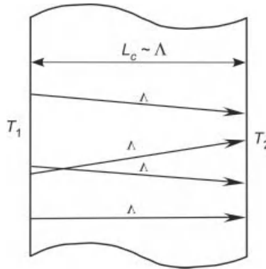
Figure 16-6 Casimir limit for ballistic transport of phonons.
