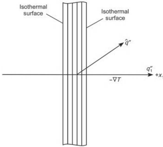
Figure 15-1 Heat flow across a large thin crystal plate.
