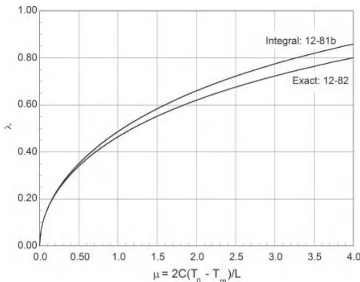
Figure 12-8 Comparison of exact and approximate solutions of the melting problem in half-space.
