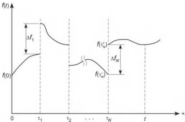
Figure 7-2 Boundary condition function f(t) with discontinuities.
