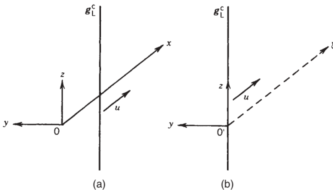
Figure 11-2 Moving line heat source: (a) fixed coordinates x, y and (b) moving coordinates \xi, y .
