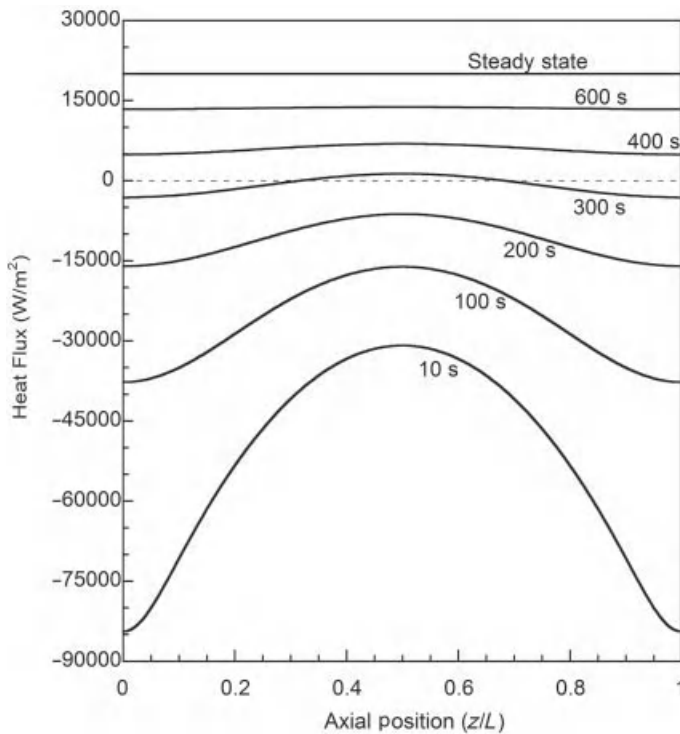
Figure 4-8 Radial heat flux at the surface r = b as a function of axial position for various times and at steady-state conditions.
