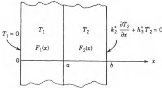
Figure 10-5 Two-layer slab in perfect thermal contact at interface.
