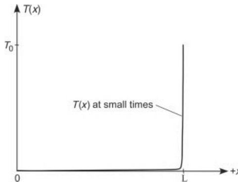
Figure 9-4 Steep gradients near the surface yield poorly convergent solutions for small times.
