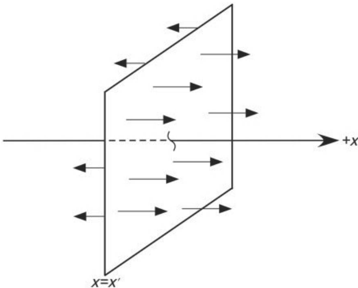
Figure 8-2 One-dimensional planar heat source in Cartesian system.
