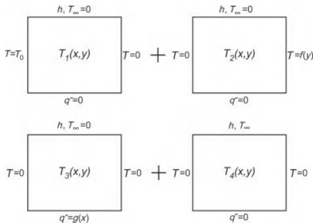
Figure 3-12 Superposition scheme for Example 3-5.
