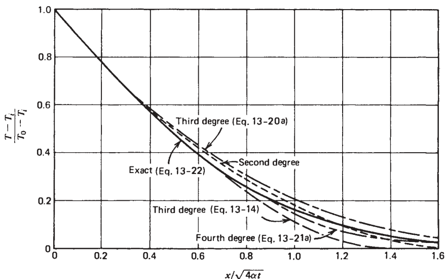
Figure 13-3 Comparison of exact and approximate analytical solutions for a semi-infinite region.
