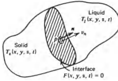
Figure 12-2 Solidification in three dimensions. Interface is moving in the direction of the surface normal n .
