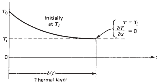
Figure 13-1 Definition of thermal penetration layer for heat conduction in a semi-infinite medium.
