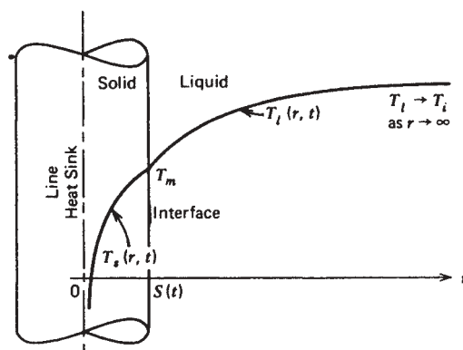
Figure 12-6 Solidification by a line heat sink in an infinite medium with cylindrical symmetry. Two-phase problem.
