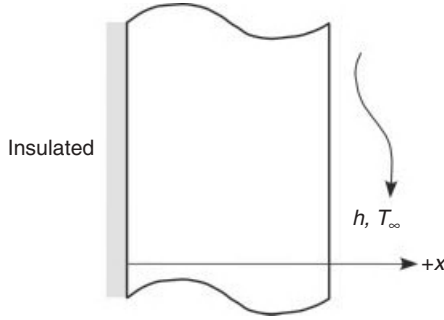
Figure 3-2 Transient heat conduction in a slab.
