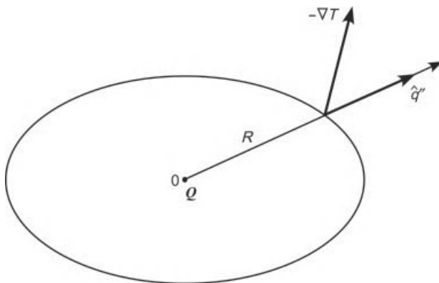
Figure 15-3 Ellipsoidal isothermal surfaces around a point source, Q .
