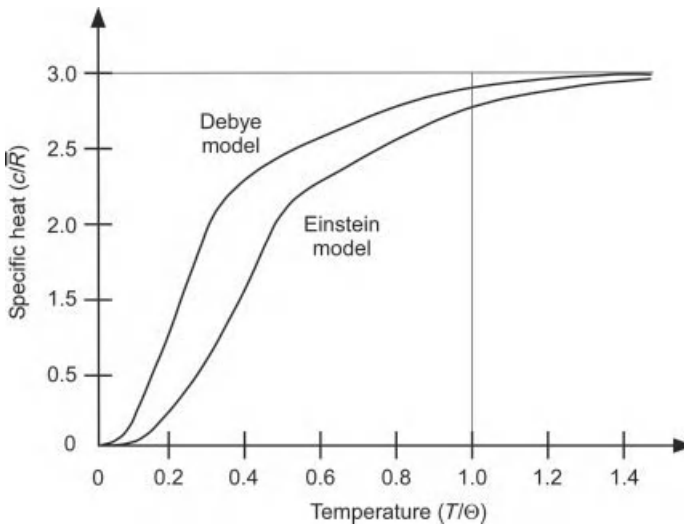
Figure 16-4 Idealized behavior of the specific heat for vibrational energy storage in crystalline materials.
