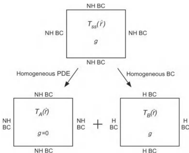
Figure 3-8 Superposition for general steady-state problem.
