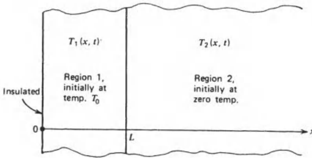
Figure 10-7 Finite and semi-infinite regions in perfect thermal contact.
