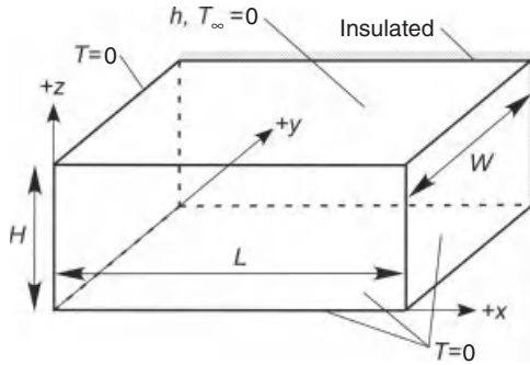
Figure 3-6 Problem description for Example 3-4.
