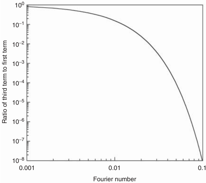
Figure 3-19 Convergence of the ratio of third-to-first terms.
