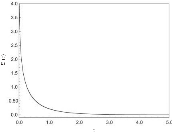
Figure 12-7 Exponential integral function E_1(z) .
