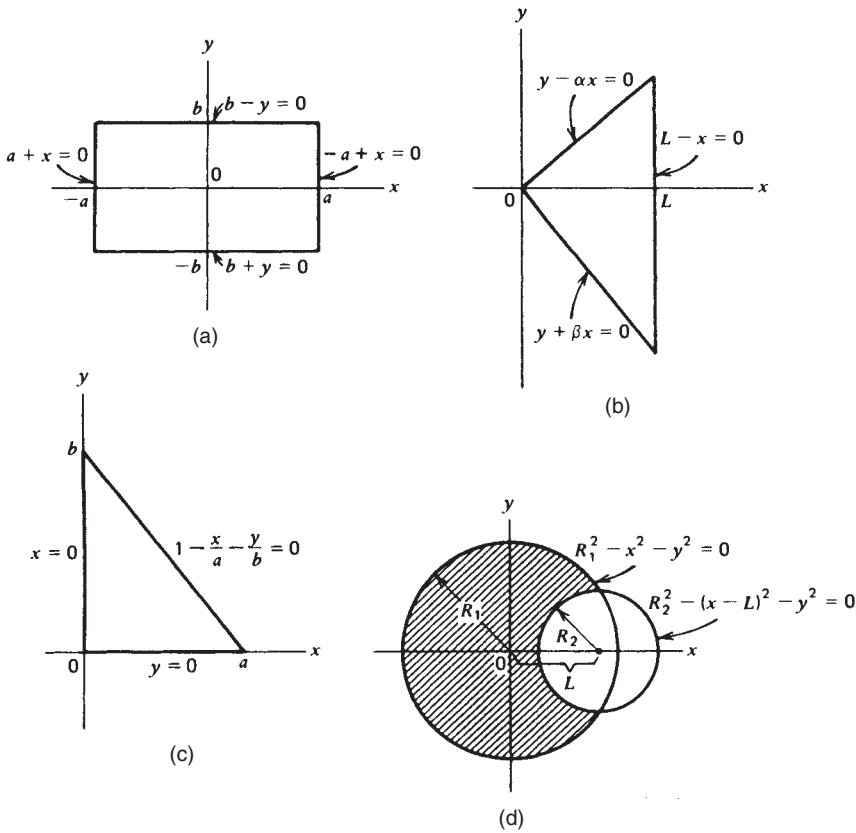
Figure 13-8 Regions having boundary contour in the form of a convex polygon and a region bounded by two circles: (a) rectangular region, (b) triangular region, (c) triangular region, and (d) a crescent-shaped region between two intersecting circles.
