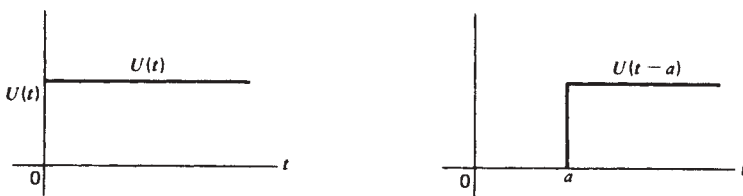
Figure 9-1 Definition of the unit-step functions U(t) and U(t-a) .
