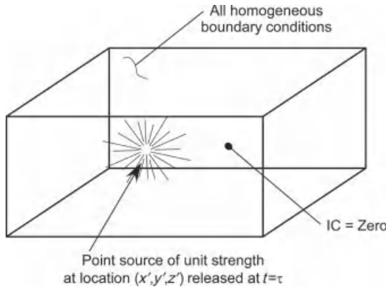
Figure 8-1 Physical problem statement for Green's function.
