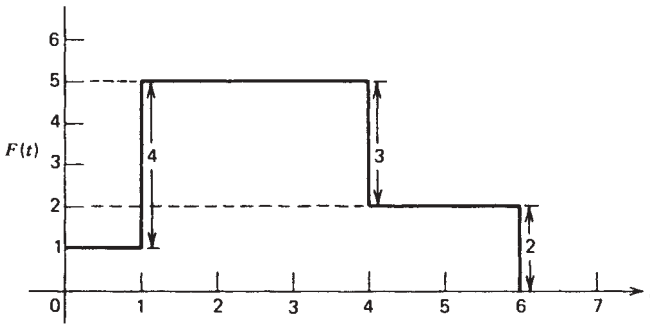
Figure 9-3 Function defined by equation (9-29).
