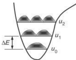
Figure 16-3 Vibrational quantum well showing discrete energy levels.
