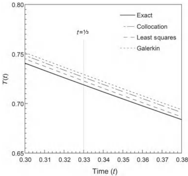
Figure 13-7 Closeup of Figure 13-6 showing the four solutions in the vicinity of t = \frac{1}{3} .
