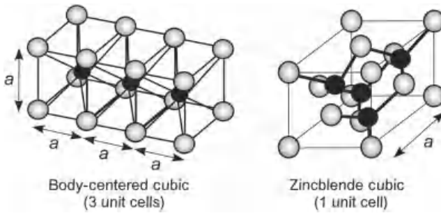
Figure 16-2 Unit cell structures.
