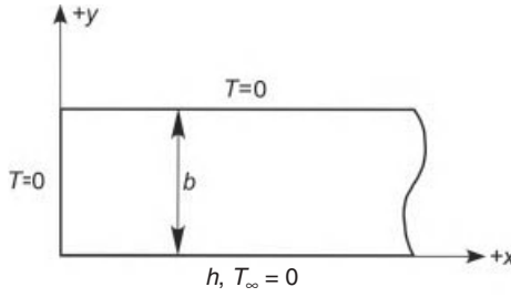
Figure 6-3 Problem description for Example 6-3.
