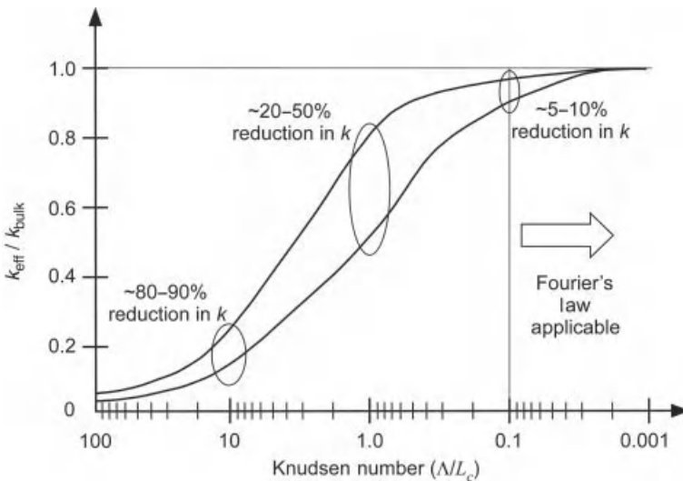
Figure 16-7 Range of effective thermal conductivity as a function of the Knudsen number.
