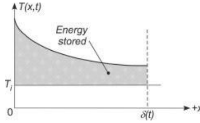
Figure 13-2 Conservation of energy associated with the energy integral equation.
