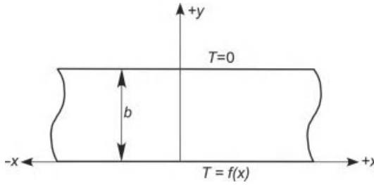
Figure 6-6 Problem description for Example 6-7.
