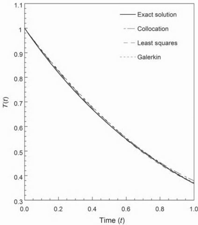
Figure 13-6 Comparison of the exact solution [equation (13-82)] with the collocation [equation (13-88)], the least-squares [equation (13-91)], and the Galerkin [equation (13-95)] solutions over the full domain of the problem.
