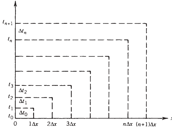
Figure 12-10 Subdivision of x - t domain using constant \Delta x , variable \Delta t .
