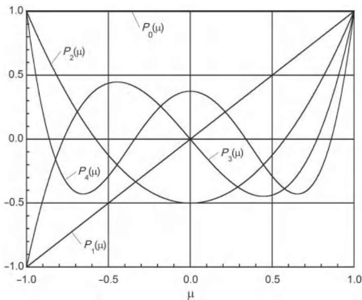
Figure 2-3 First five Legendre polynomials of the first kind P_n(\mu) .
