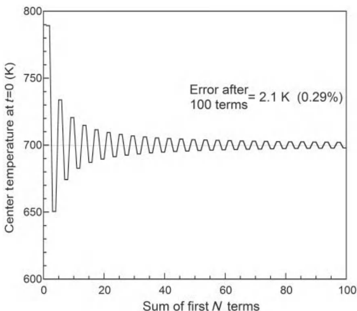
Figure 3-18 Convergence of the center temperature at t = 0 .
