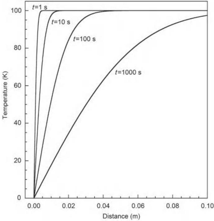
Figure 6-2 Behavior of 1-D semi-infinite solution of equation (6-39).
