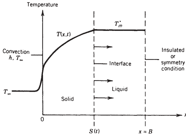
Figure 12-9 Geometry and coordinate for single-phase solidification.
