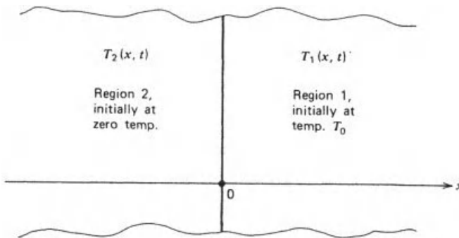
Figure 10-6 Two semi-infinite regions in perfect thermal contact.
