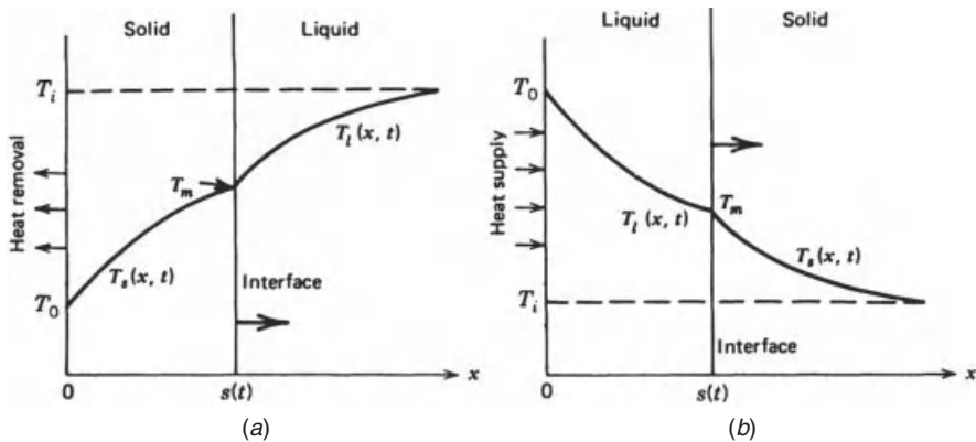
Figure 12-1 Geometry and coordinates for one-dimensional (a) solidification and (b) melting problems.
