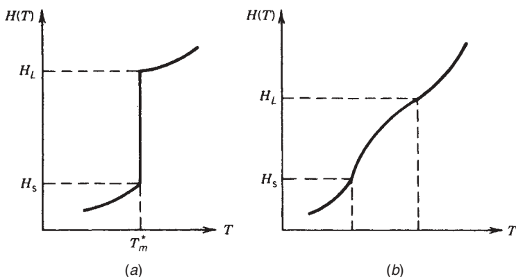
Figure 12-11 Enthalpy–temperature relationship for (a) pure crystalline substances and eutectics and (b) glassy substances and alloys.
